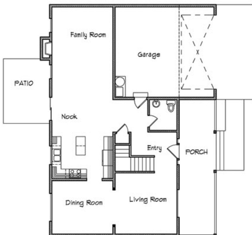
MAIN LEVEL
