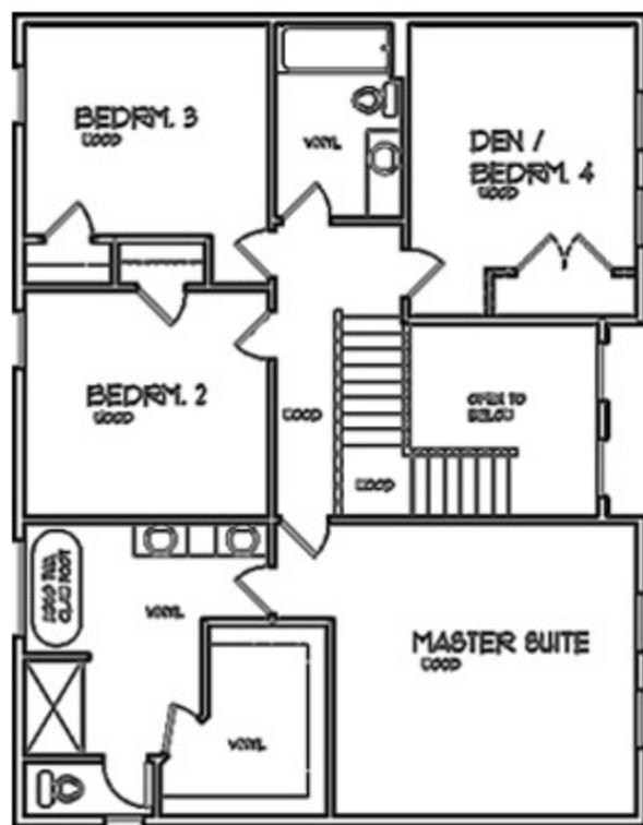
UPPER LEVEL
