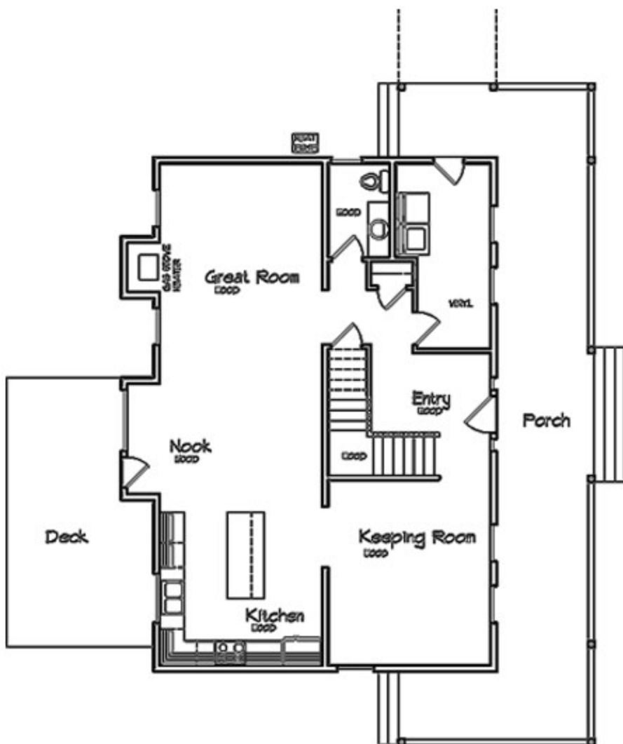
MAIN LEVEL
