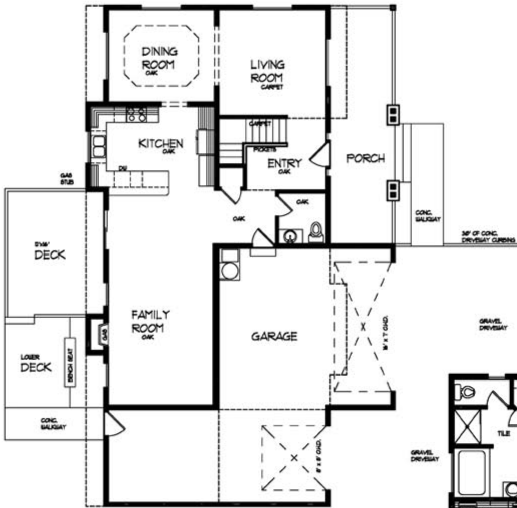
MAIN FLOOR
